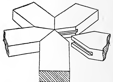
FIG. 558. JOINT OF FIVE-SPOKE SPIDER.
